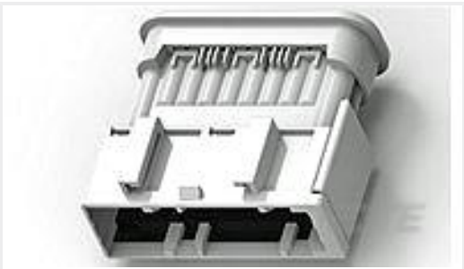
TE 产品编号179228-4 CT CRIMP-2 REC HSG 4P NATURAL
