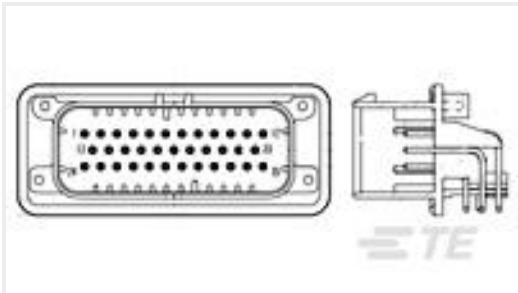
TE 产品编号1-776163-4 35POS,AMPSEAL,PIN HSG ASSY,SLD, COD 4
