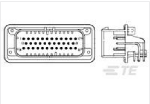
TE 产品编号776163-1 35POS,PIN DIA 1.3,HDR ASSY,90DEG, COD 1
