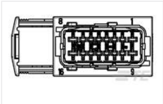
TE 产品编号185760-2 16W HYBRID RCPT HSG GREEN
