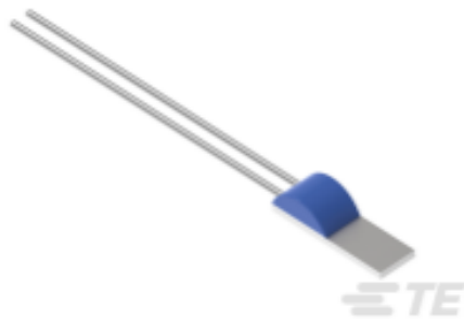
TE 产品编号NB-PTCO-192 Pt1000, 1.2x4.0, Class A, PTFM102A1A0
