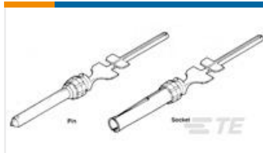
TE 产品编号5-745288-5 20 DF SKT CONTACT DUPLEX/LP
