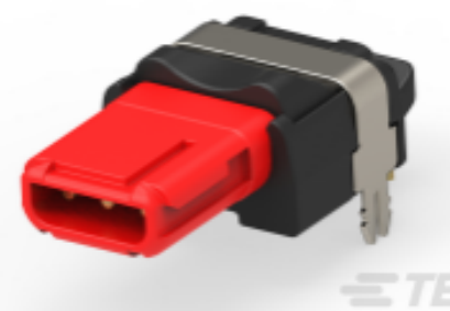
TE 产品编号 CAT-D369-G33 PCB Mount Receptacle: 3-Way Inline
