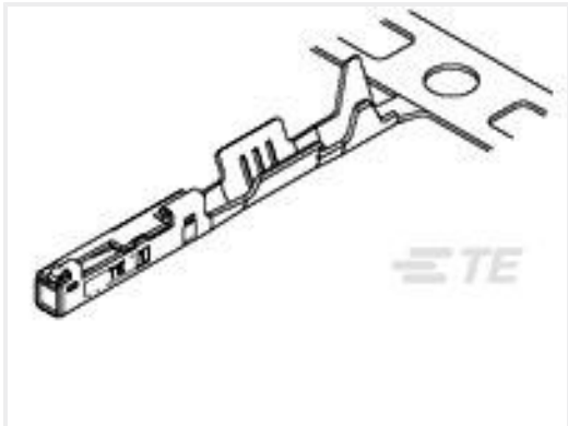
TE 产品编号1827855-4 0.50 SERIES CONNECTER RECEPTACLE CONTACT
