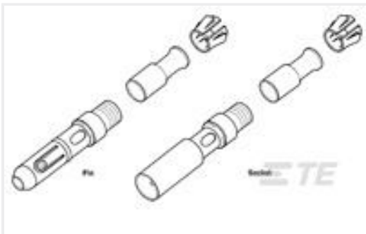
TE 产品编号9-328666-3 FERRULE, STEP DOWN, PLTD
