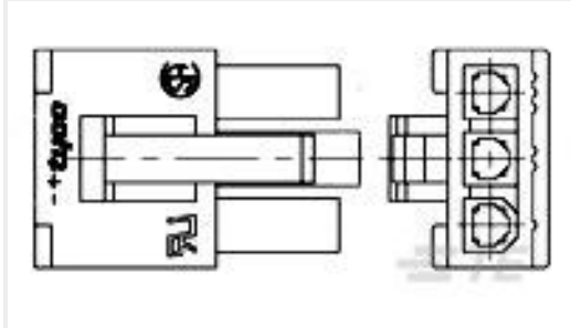
TE 产品编号1586027-5 5P SR RCPT VAL-U-LOK V0
