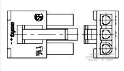
TE 产品编号1586027-4 4P SR RCPT VAL-U-LOK V0
