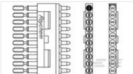
TE 产品编号699219-000 MTCB2X-XXX-205
