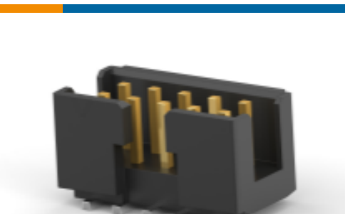
TE 产品编号1-2373376-0 10P,2MM,SHRD HDR,DRVT,SMD,0.1 AU,TB
