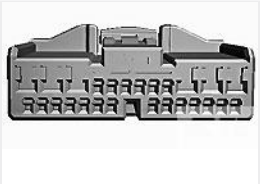
TE 产品编号1674932-1 0.64 III/2.3 II 26POS PLUG ASSY
