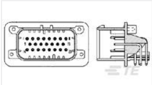
TE 产品编号1-776267-1 14POS,PIN DIA 1.3,HDR ASSY,90DEG, COD 1
