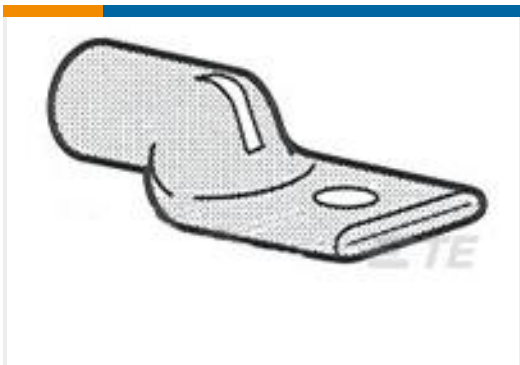
TE 产品编号325605 TERMINAL,AMPPOWER 4/0 1/2
