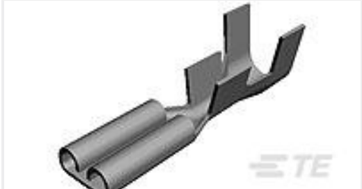
TE 产品编号41202 250 FASTON, REC., 18-14 AWG, BR
