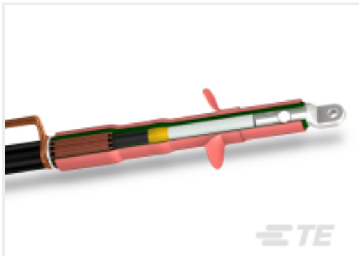
TE 产品编号CF6305-070 POLT-42E/1XO-ML-5-13
