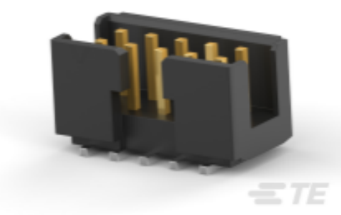
TE 产品编号1-2373376-0 10P,2MM,SHRD HDR,DRVT,SMD,0.1 AU,TB
