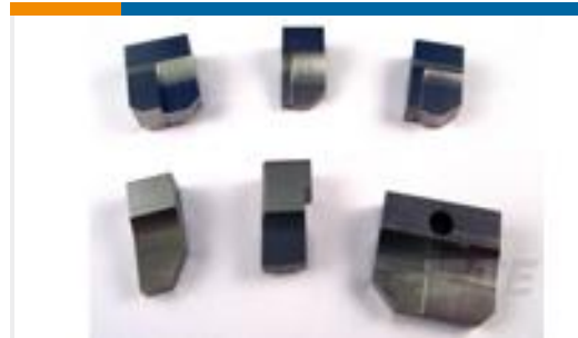
TE 产品编号1-1333225-1 ANVIL, COMBINATION SPECIAL
