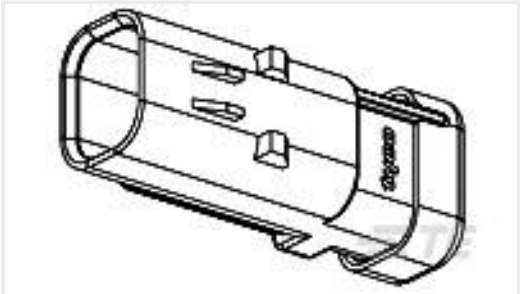
TE 产品编号776535-4 AS16,CAP ASSY,ST,03P,E SEAL,CODE D
