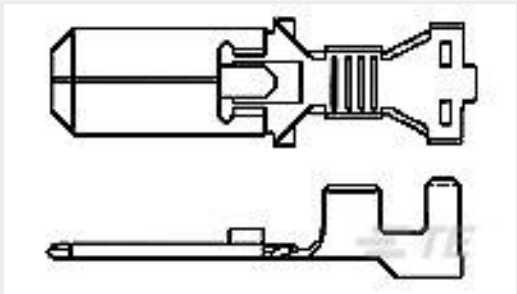
TE 产品编号344069-1 .250" SPEC. F.TAB.(PLATED)
