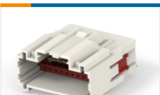
TE 产品编号2-2208018-2 22POS,0.64 MALE GEN. Y, PIN HSG, ASSY
