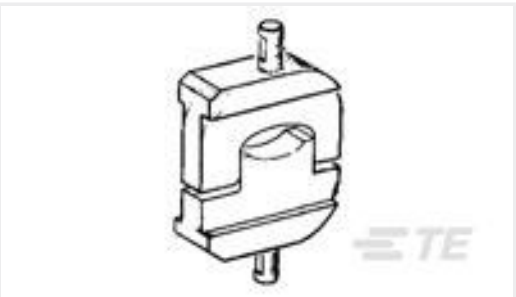
TE 产品编号45442 HYP8/10 SOLIS 3/0AWG DIE SET
