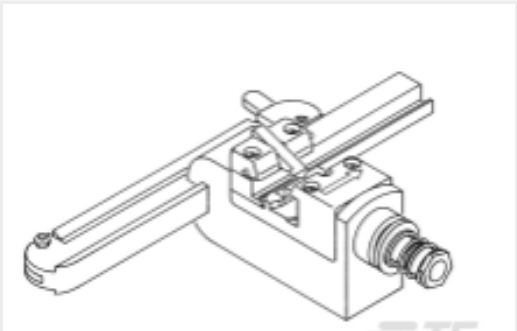
TE 产品编号58442-1 MTA 100 CRIMP HEAD PRODUCTION FEED THRU
