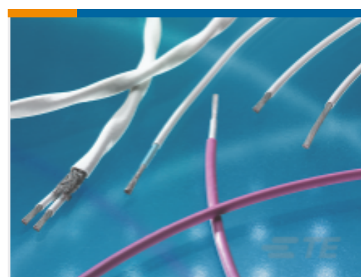
TE 产品编号 CAT-55PC-S-2T-8-18 2 Core Twisted Pair Cable: Silver Coated Cable, 8-18 AWG
