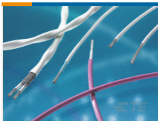
TE 产品编号 CAT-55A-SC-2T16 General Purpose 2 Core Cable: Silver Coated Copper, 16 AWG
