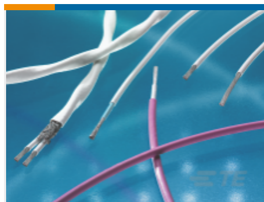
TE 产品编号 CAT-55A-S-3T-16-20 General Purpose 3 Core Cable: Silver Coated Copper, 16-20 AWG
