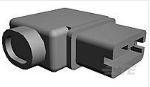
TE 产品编号180429-1 250 FASTON,FLAG,REC.,17-14 AWG, BR
