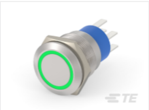
TE 产品编号5-2213767-3 AV19 DPM 3A MOVE RING LED GREEN 12V
