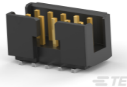
TE 产品编号1-2373376-0 10P,2MM,SHRD HDR,DRVT,SMD,0.1 AU,TB
