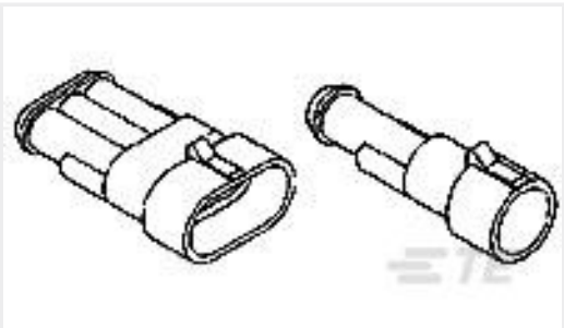
TE 产品编号282108-1 AMP SUPERSEAL 1.5 SERIES 6P CA
