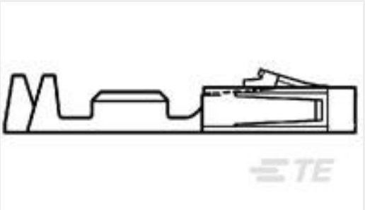
TE 产品编号1-104480-4 SHORT POINT RECP CONT LP
