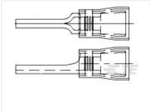
TE 产品编号696394-2 TERM, WIRE PIN, PIDG, 16-14, T&R
