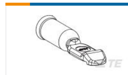
TE 产品编号647879-1 SERIES 50&75 CONTACT,10-12 AWG
