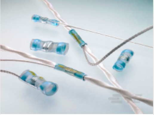
TE 产品编号EJ3514-000 S200-3-55-22-9CS2904
