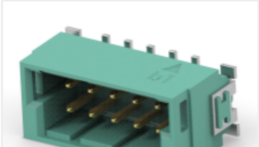
TE 产品编号474008-E DRCQ 2,54 10 M * SMD * 137 E012 167 GU-H
