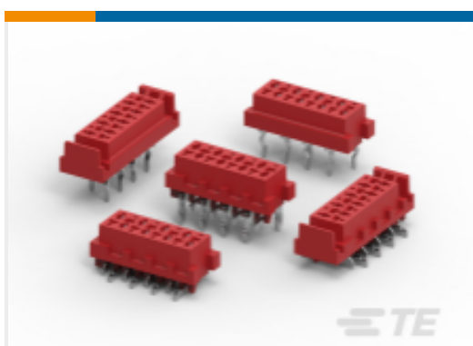
TE 产品编号8-215079-2 Female-on-Board Connector, Top Entry
