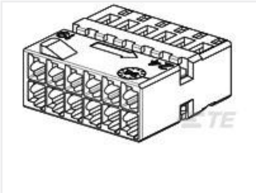
TE 产品编号1-968318-1 12POS MQS REC COD A
