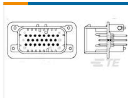
TE 产品编号776228-5 23POS,PIN DIA 1.3,HDR ASSY, 180DEG,COD 5
