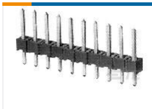
TE 产品编号826938-4 4P AMPMODU II STIFT LEI
