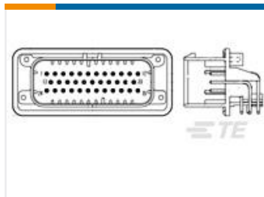
TE 产品编号776163-4 35POS, PIN DIA 1.3, HDR ASSY, 90DEG, COD 4
