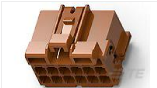
TE 产品编号3-967624-6 JUN-POW-TIM GEH 18P
