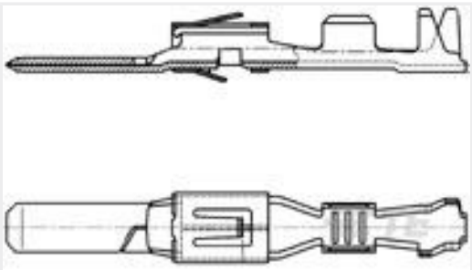
TE 产品编号962882-2 TAB AS 2.8x0.8 CONTACT CF SRC Sn
