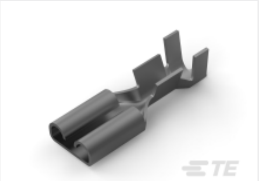
TE 产品编号5-160493-2 187 FASTON REC 20-16 AWG TPBR
