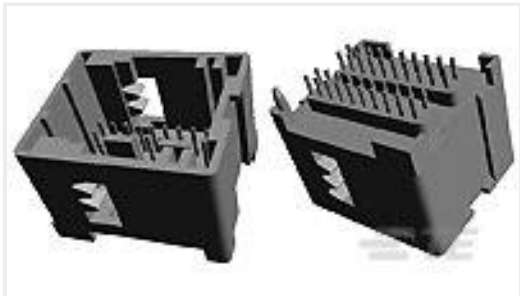
TE 产品编号953118-1 40pos MQS .63 header 180deg
