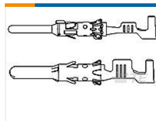
TE 产品编号1703013-1 DIA 1.5MM CONTACT PIN, ASSY
