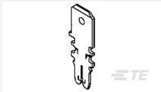
TE 产品编号1217497-1 TAB,187FASTON,MAG-MATE,SLIMLIN
