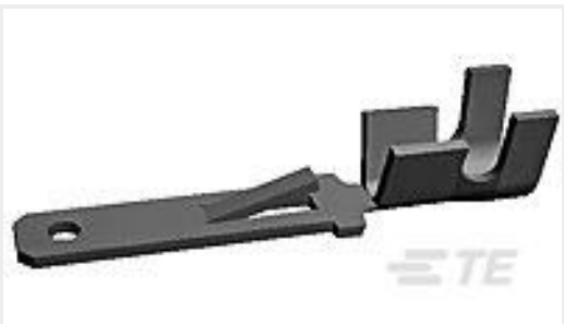
TE 产品编号60294-2 FF 250 TAB 22-18 AWG .032 TPBR
