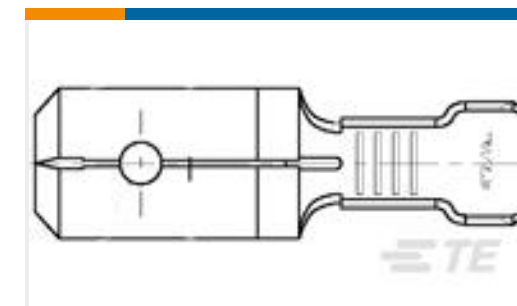
TE 产品编号60006-2 250 FASTON TAB 18-14 AWG TPBR
