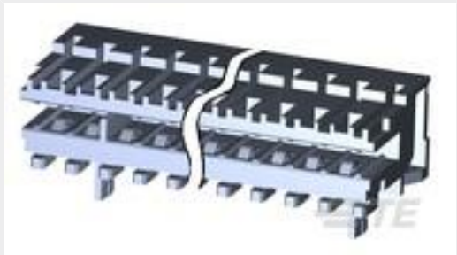
TE 产品编号1-282044-1 AMP MONO-SHAPE P.C.B.CONN4P. G
