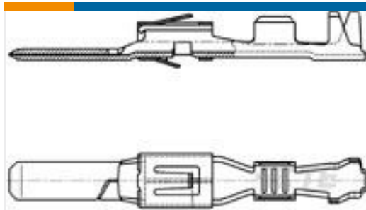
TE 产品编号962884-1 TAB AS 2.8x0.8 CONTACT CS SRC Sn
