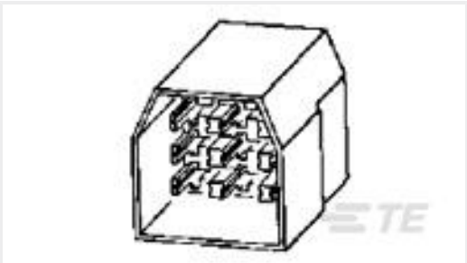
TE 产品编号151326-1 FF 250 TAB HSG 11P NYLON NAT
