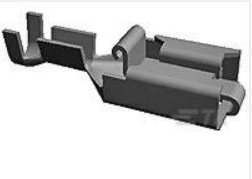
TE 产品编号154718-4 PL 250 REC TERMINAL 17-15 AWG TPPB
